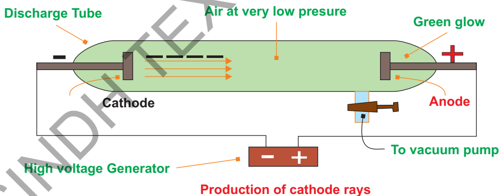
Fig (2.6) William Crooks Discharge Tube
