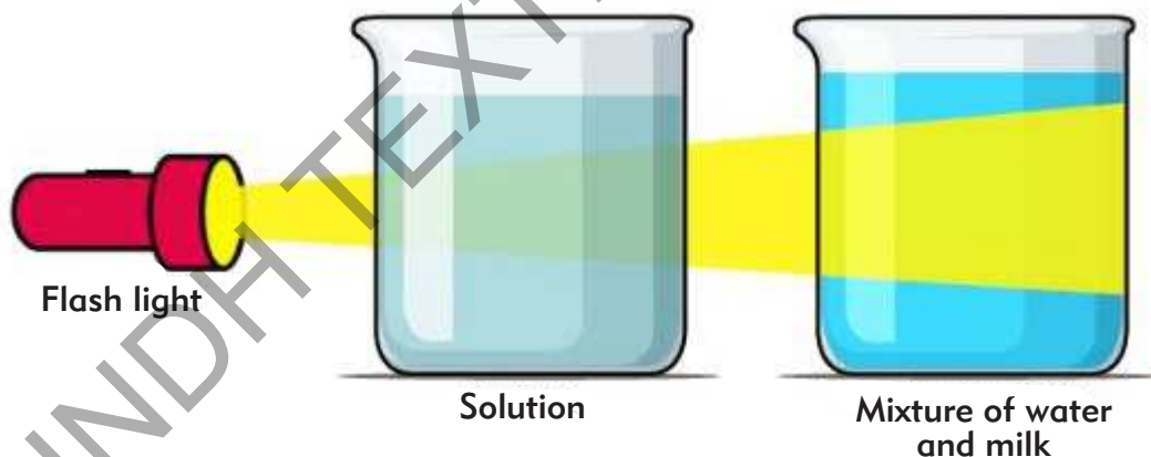
Figure: 6.3 Tyndall effect by colloids
