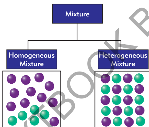
Fig 1.5 Types of Mixture
