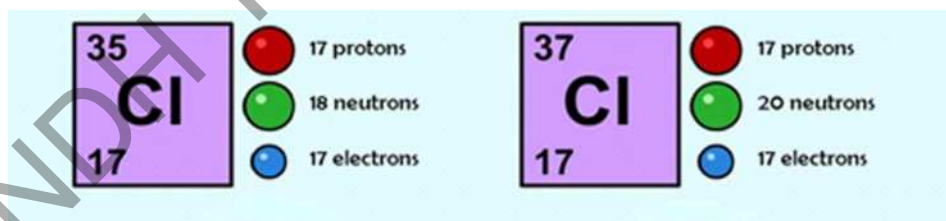
Fig 2.23 Isotopes of Chlorine
