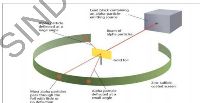
Fig 2.10 Gold Foil experiment
