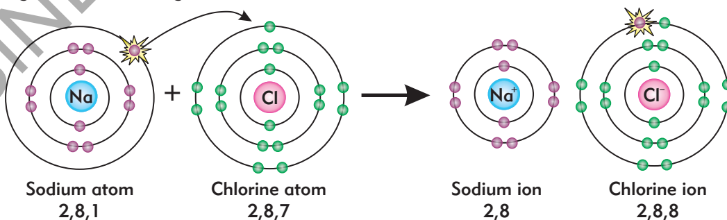
Fig 4.3 Formation of ionic bond in Sodium chloride
