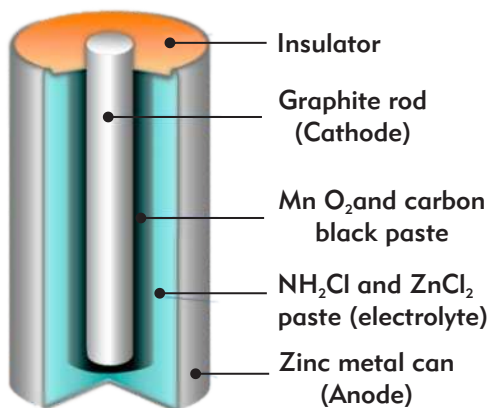
Fig 7.6 Dry cell
