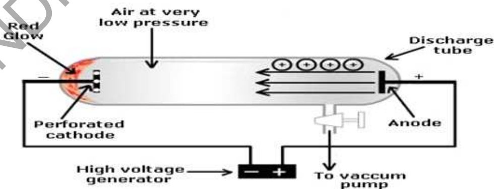
Fig 2.8 Gold Stein Discharge Tube
