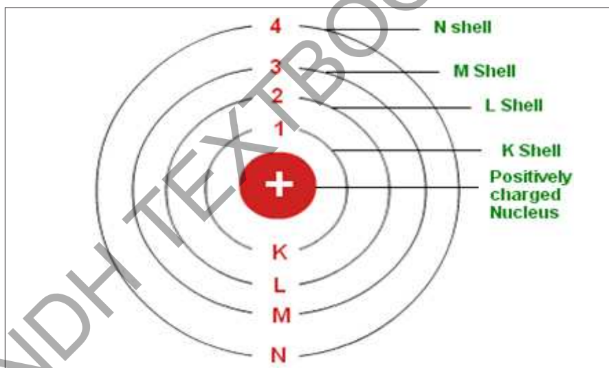
Fig 2.17 Shell (Energy level)
