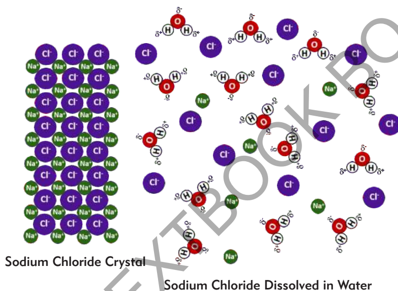
Figure 6.2 Interaction of sodium chloride and water
