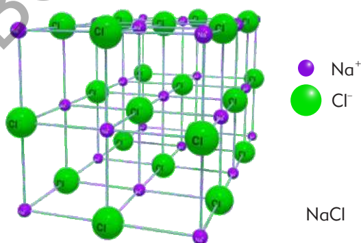
Figure 4.22 arrangement of ions in Solid crystal of NaCl
