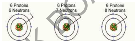
Fig 2.22 Isotopes of Carbon
