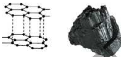
Fig 5.20 Allotropy of Graphite
