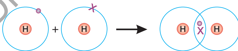
Fig 4.4 The formation of a hydrogen molecule
