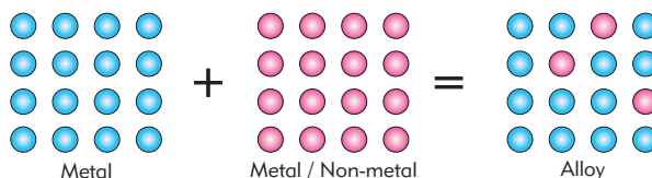
Fig 7.8 Alloy formation
