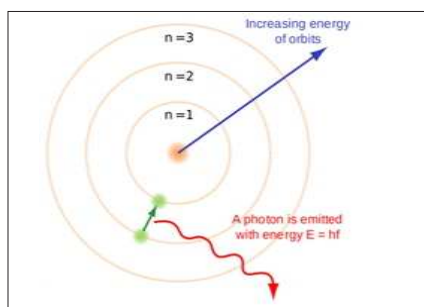
Fig 2.13 Neil Boher's Atomic model
