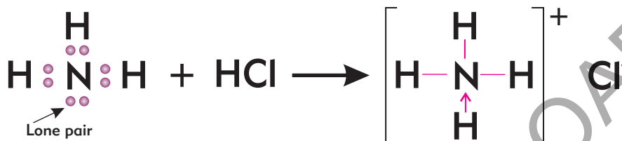
Fig 4.9 Reaction between Ammonia and Hydrogen Chloride
