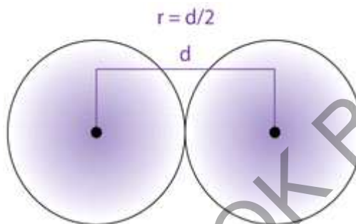
Fig 3.4 Atomic radius
