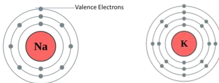
Fig 3.5 Shielding effect in Potassium atom is more than Sodium atom
