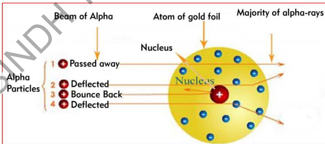
Fig 2.11 Pictorial description of bombardment of alpha particles on gold foil
