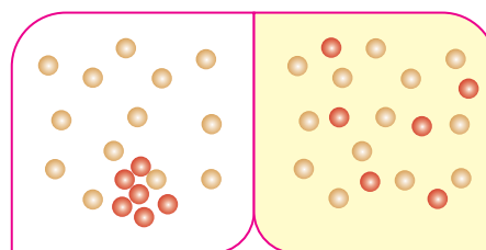
Fig 5.2 Gharam's Law of diffusion
